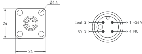
4 pin Male Connector Configuration
